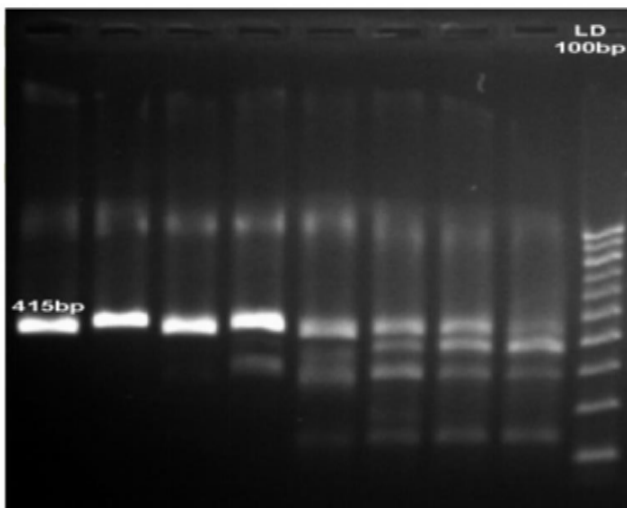
Figure 1. Electrophoresis of GTADIANT PCR results on DNA bands resulting from Real-Time PCR optimization.
